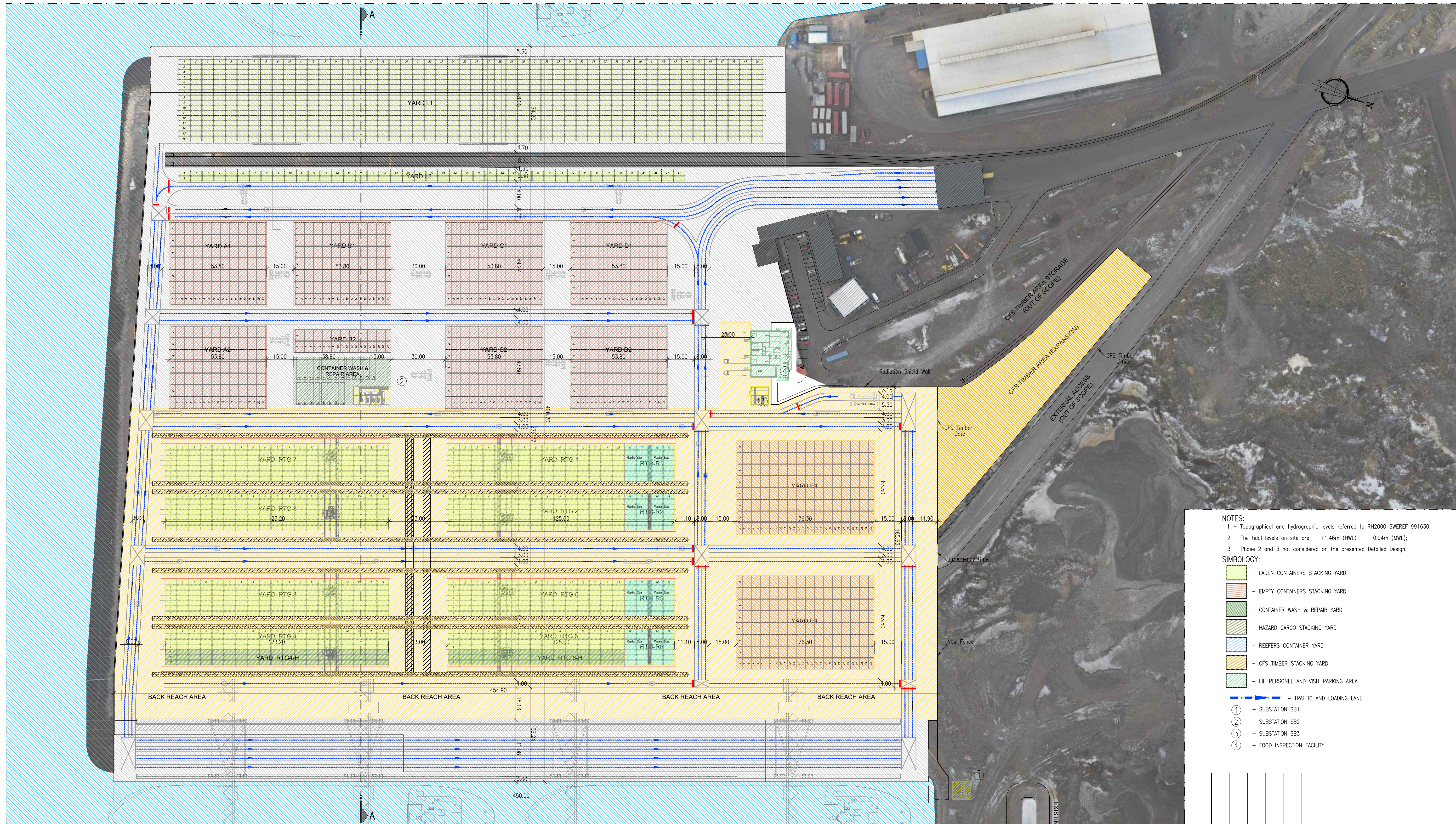
General Plan
